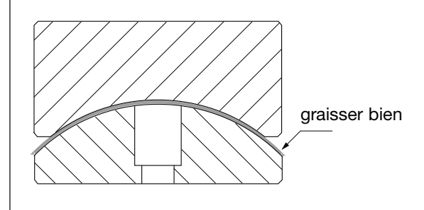
illustration 2 - Tête oscillante CAT
